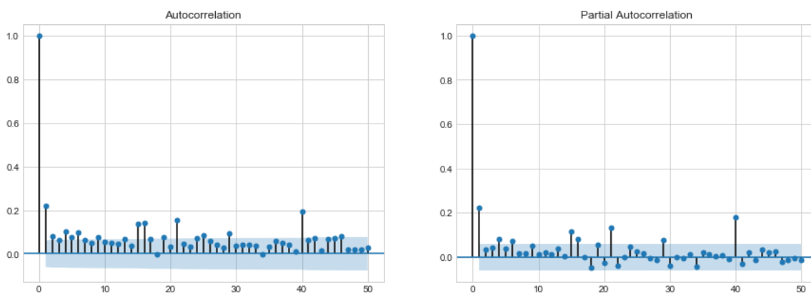
Figure 16: Autocorrelation plot of the model residuals squared
