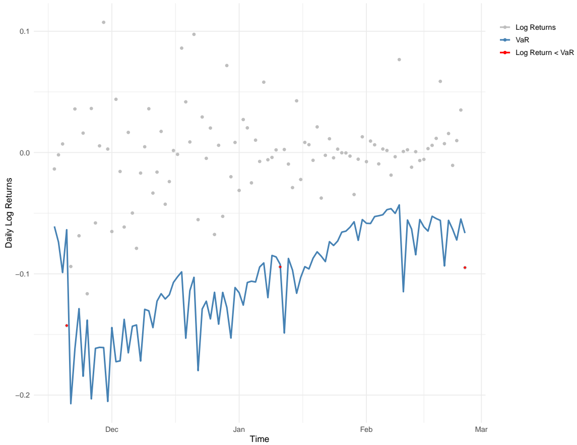
Figure 18: 95% Value-at-Risk forecast using a rolling window of 100 days
