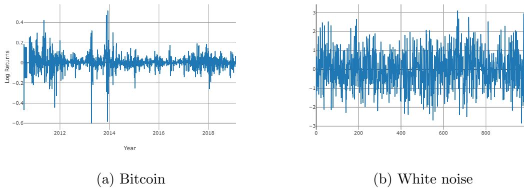
Figure 8: Difference in log returns
