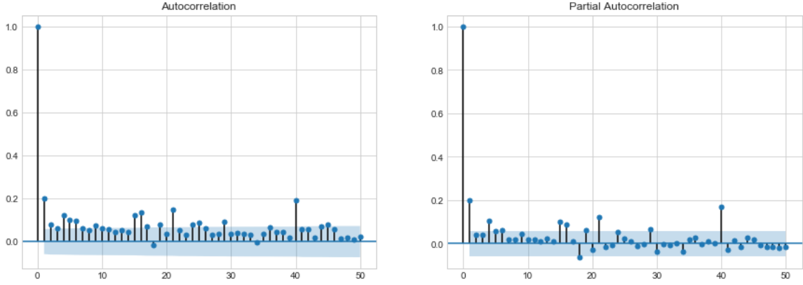
Figure 15: Autocorrelation plots of the squared BTC log returns
