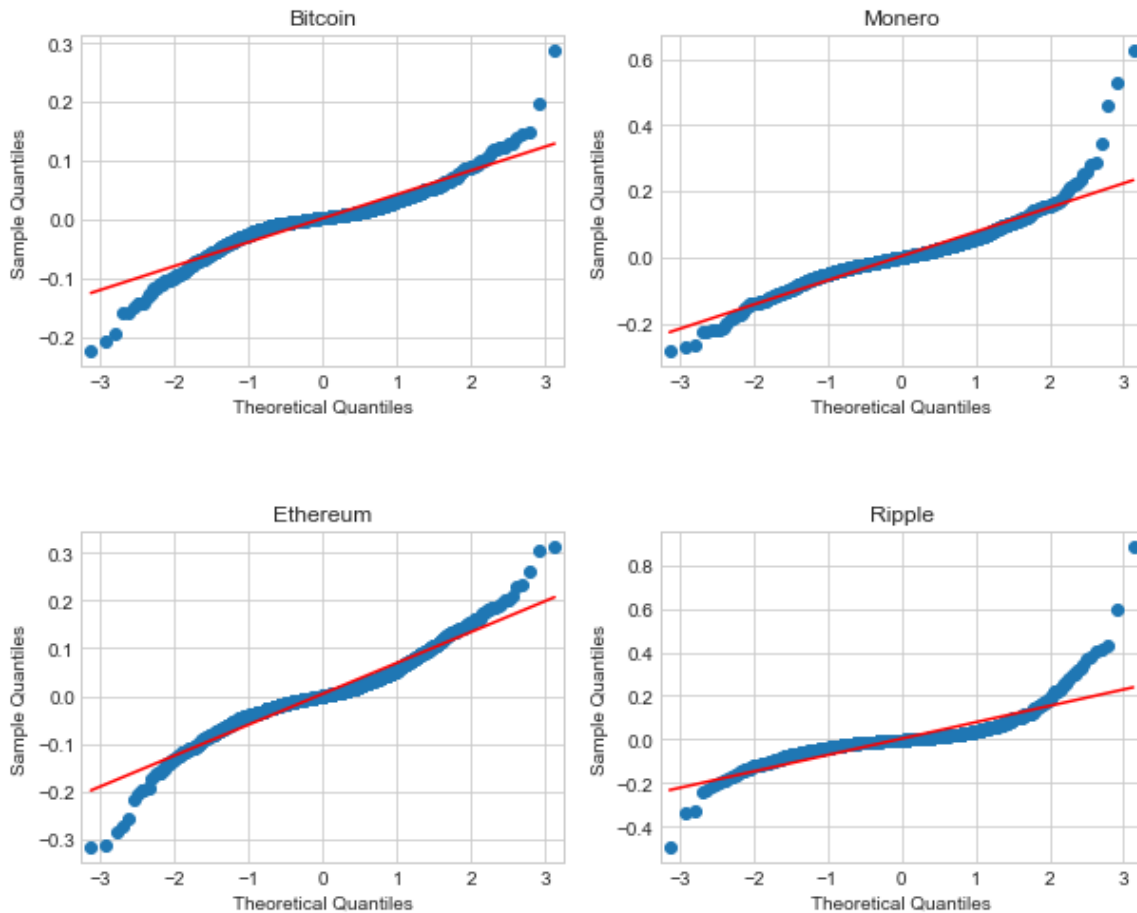
Figure 9: Quantile-quantile plot of log returns of different cryptocurrencies
