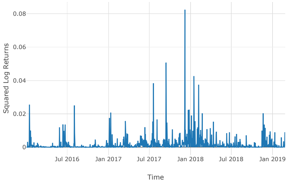
Figure 13: Squared log returns of Bitcoin
