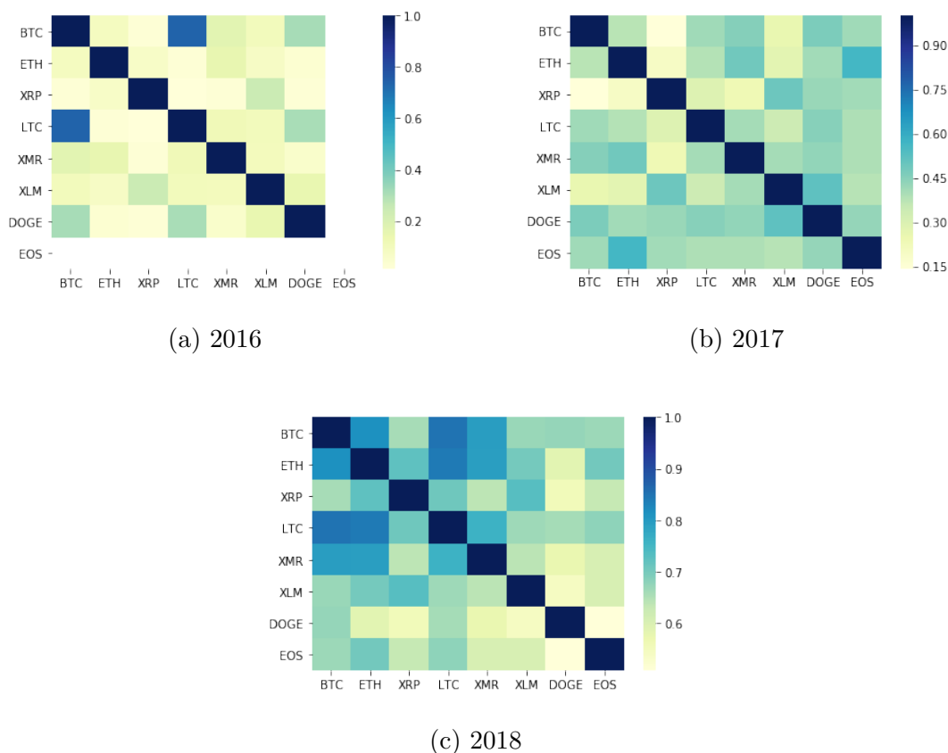
Figure 4: Correlation heatmaps between different cryptocurrencies through the years.
