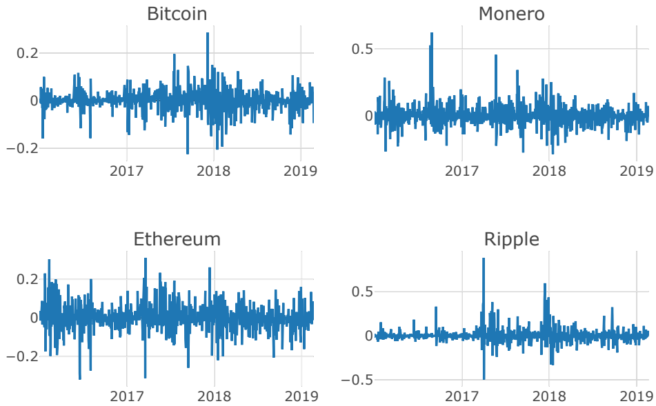
Figure 1: Log returns of the different cryptocurrencies
