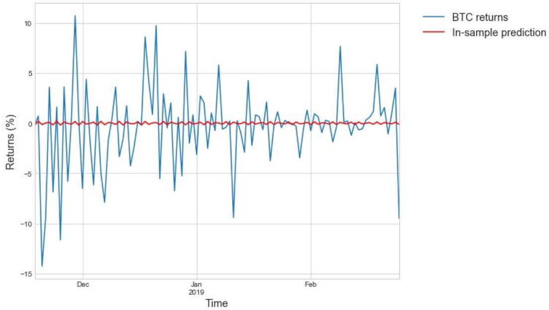
Figure 17: Mean-process of the model
